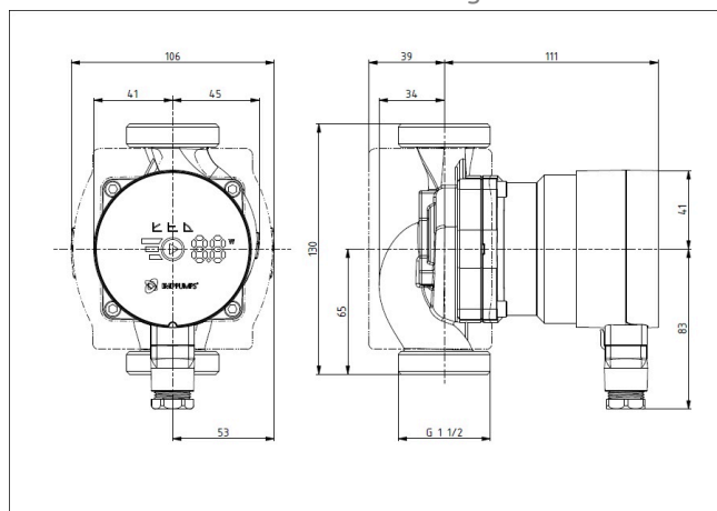
Dimension drawing
